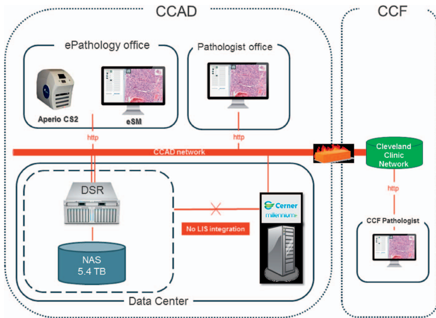
Figure 1. Architecture display of the information technology (IT) set up of ePathology at Cleveland Clinic Abu Dhabi (CCAD). Abbreviations: CCF, Cleveland Clinic Foundation (Cleveland, Ohio); DSR, digital slide repository; eSM, Aperio managing software eSlide Manager (Leica Microsystems), Cerner Millennium (Cerner Corporation, Kansas City, Missouri), and Aperio CS2 scanner (Leica Microsystems); LIS, laboratory information service; NAS, network-attached storage device.
