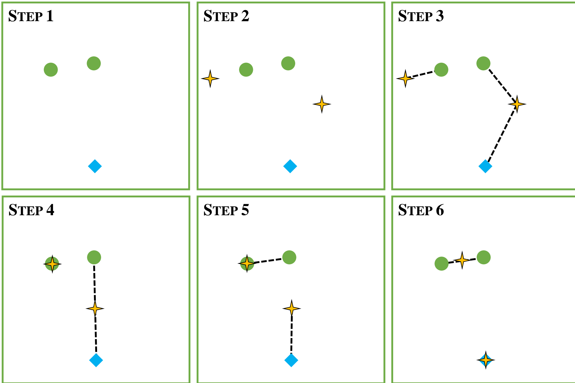
Figure S5. K-means Clustering Algorithm
