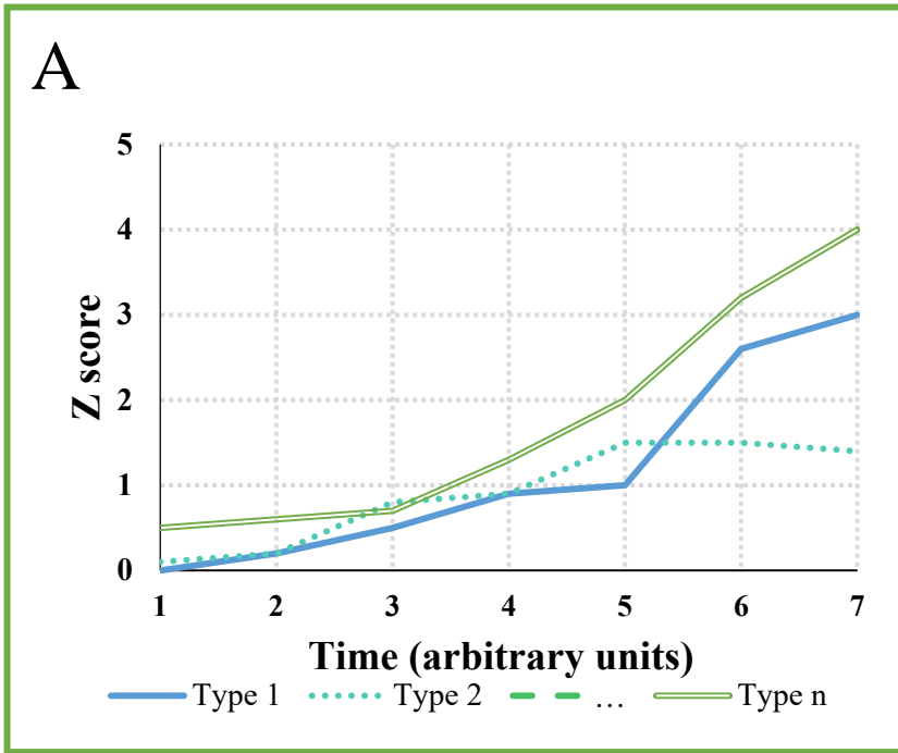
Figure S6. Subtype and Stage Inference (SuStaIn)
